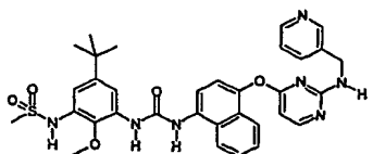
N-{5-tert-Butyl-2-methoxy-3-[3-(4-{2-[(pyridin-3-ylmethyl)amino]-pyrimidin-4-yloxy]-naphthalen-1-yl)-ureido]-phenyl}-methanesulfonamide;
